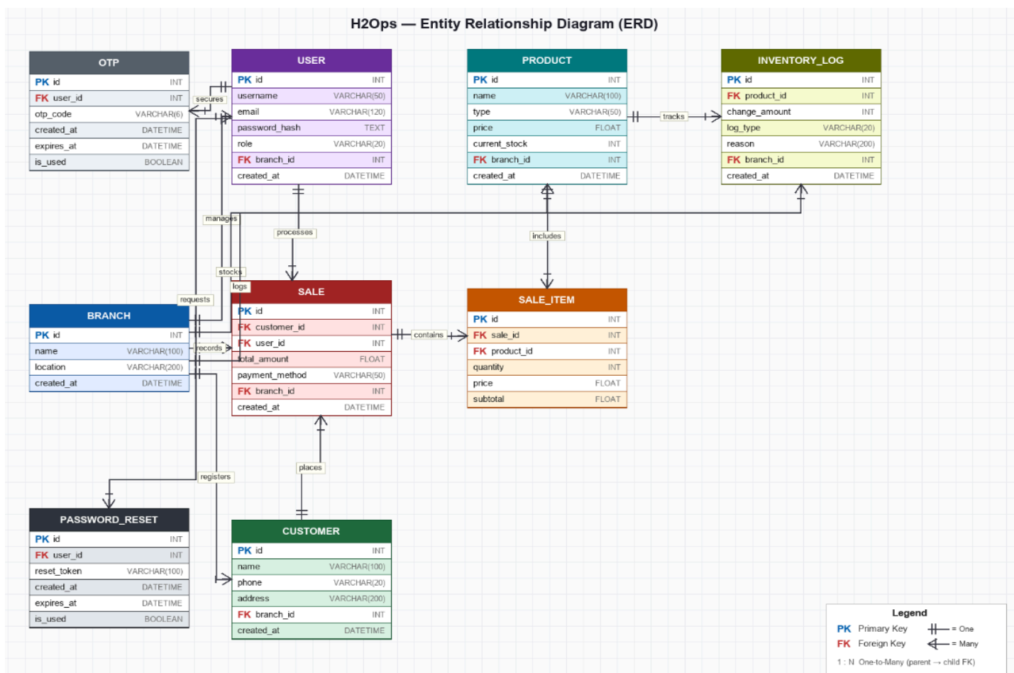
Figure 4.4 presents the Entity Relationship Diagram (ERD) of the H2Ops system.
